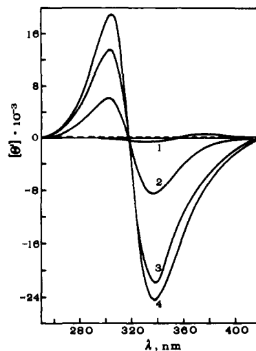
Figure 1. Poly(L-glutamic acid) containing 21 mol % azobenzene units. Time dependence of side-chain CD bands in \text{TMP}/\text{H}_2\text{O} = 50/50 . (1) Freshly prepared solution, (2) 1-day old solution; (3) 2-day old solution, (4) 3-day old solution. (—) Dark-adapted, (---) irradiated at any time. Data are expressed in terms of azobenzene molar ellipticity.
