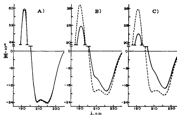
Figure 2. Poly(L-glutamic acid) containing 21 mol % azobenzene units. CD spectra in \text{TMP}/\text{H}_2\text{O} = 50/50 , recorded at various aging times. (A) Freshly prepared, (B) 1-day old, (C) 2-day old solution. (—) Dark-adapted, (---) irradiated samples. Molar ellipticity is based on the mean residue weight.
